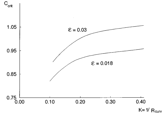
FIG. 8. The dependence of the critical velocity C_{\text{crit}} associated with the wave-front-obstacle separation on the local obstacle curvature K=1/R_{\text{curv}} for different \varepsilon . Here R_{\text{curv}} is the local curvature radius which is given by (9) and \gamma=7 , \alpha=2.76 are the medium parameters.
